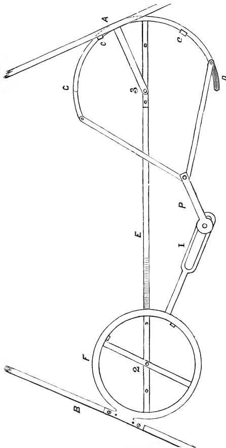
HAUSSKNECHT'S PERCH-COUPLING.
